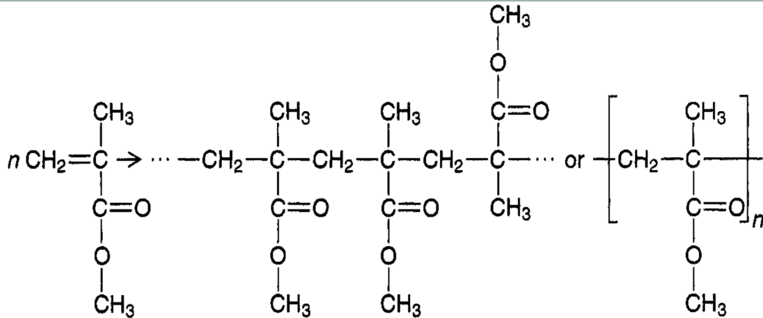
Methyl methacrylate
